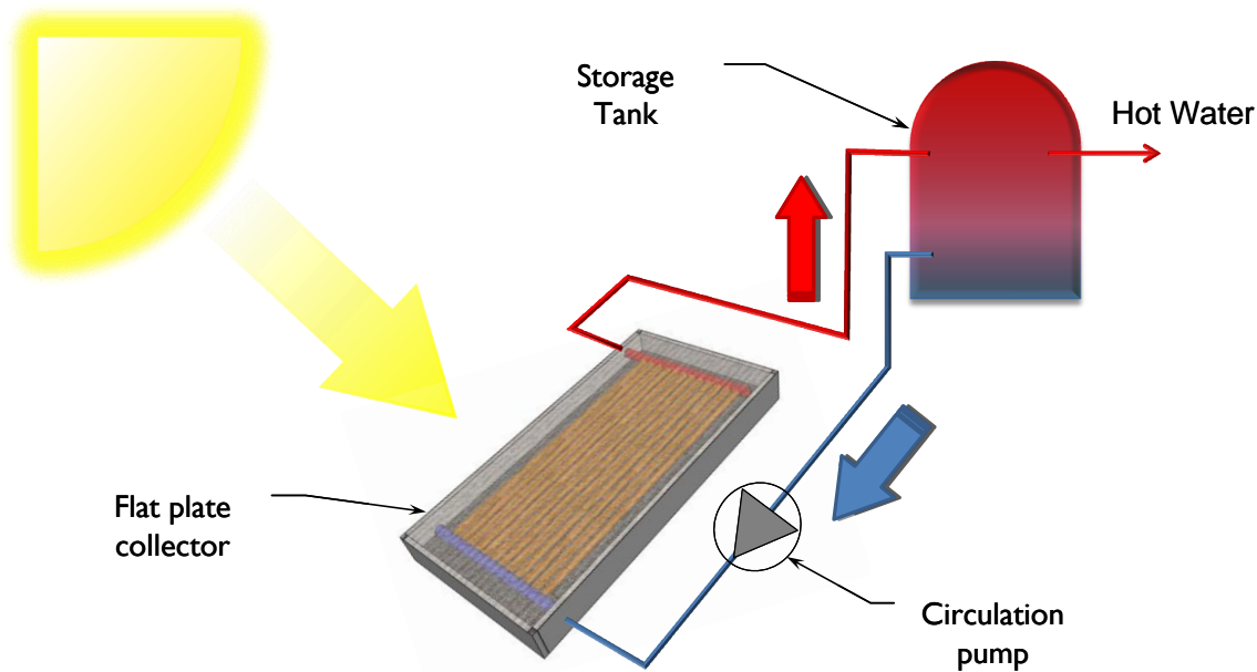
Figure 2: Active and Direct Solar Thermal System (Illustration by Author, with reference made to CIBSE Solar Heating Design and Installation Guide, 2007)
