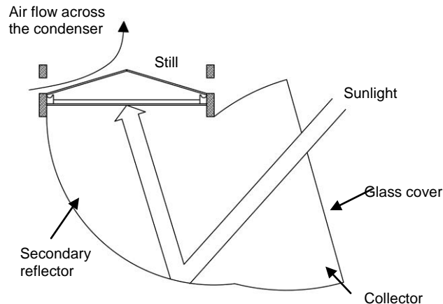
Figure 1: An inverted absorber solar still. Illustration: Neil Noble / Practical Action.
