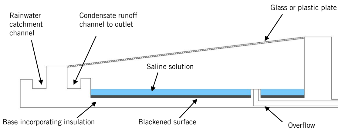
Figure 1: Shows a single-basin still. Illustration: Martin Bounds.
